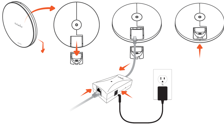
Figure 2-1: Installing the EnStation2
